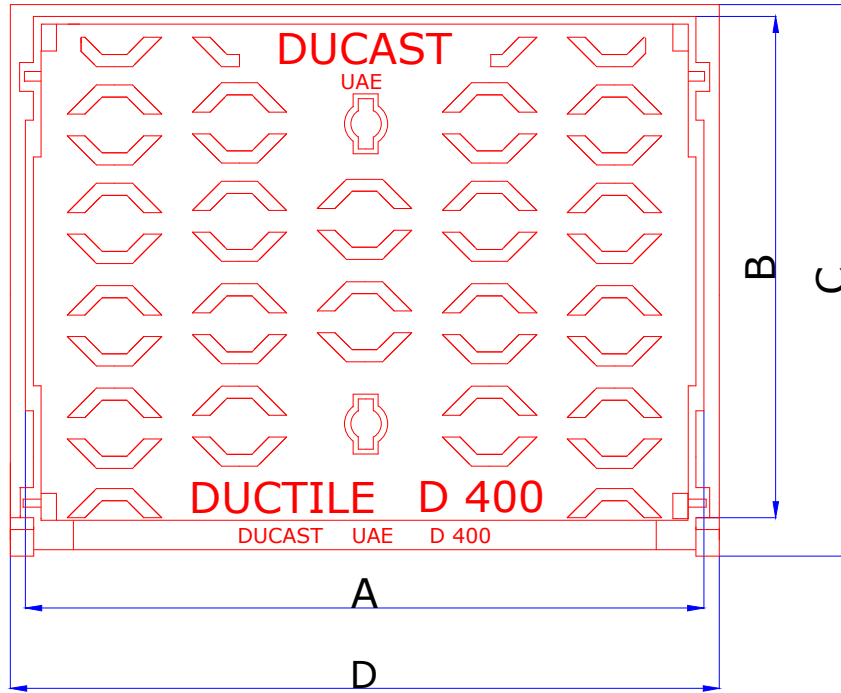
PLAN VIEW OF COVER & FRAME
