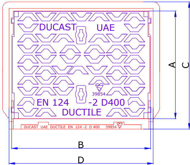
PLAN VIEW OF COVER & FRAME
