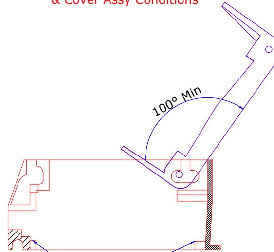
Cover opened Conditions Debris Grid Plate resting
