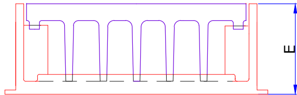
FRONT VIEW OF COVER & FRAME
