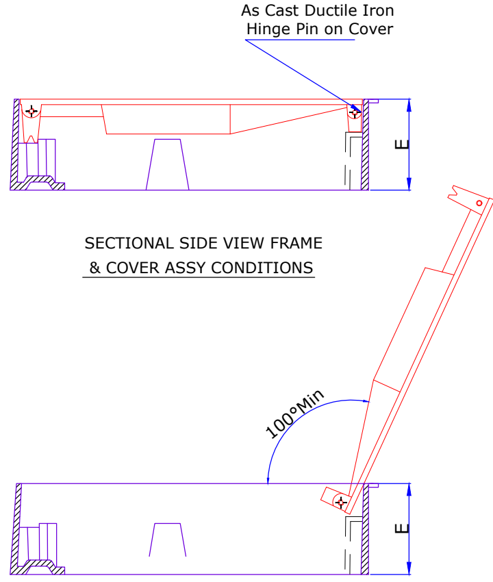
COVER OPENED CONDITIONS
