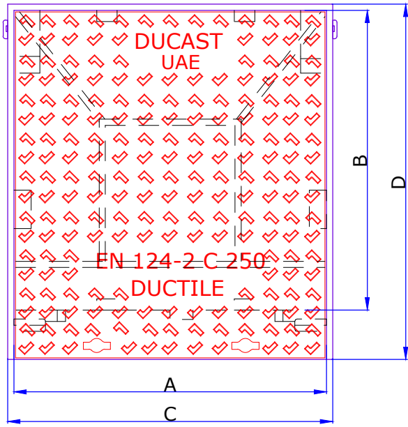
PLAN VIEW OF COVER & FRAME
