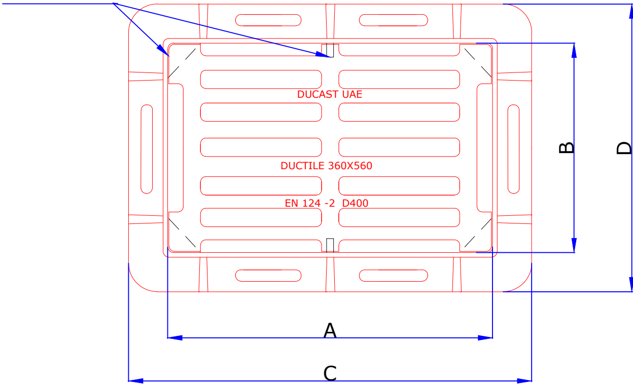
Plan View of Grating & Frame
