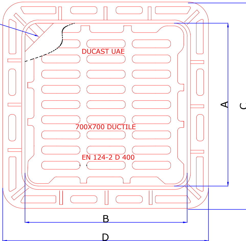
PLAN VIEW OF GRATING & FRAME
