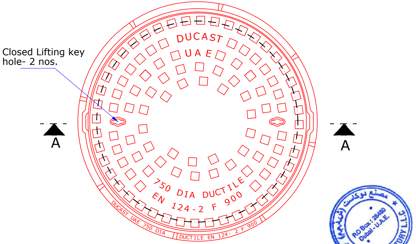
PLAN VIEW OF COVER & FRAME
