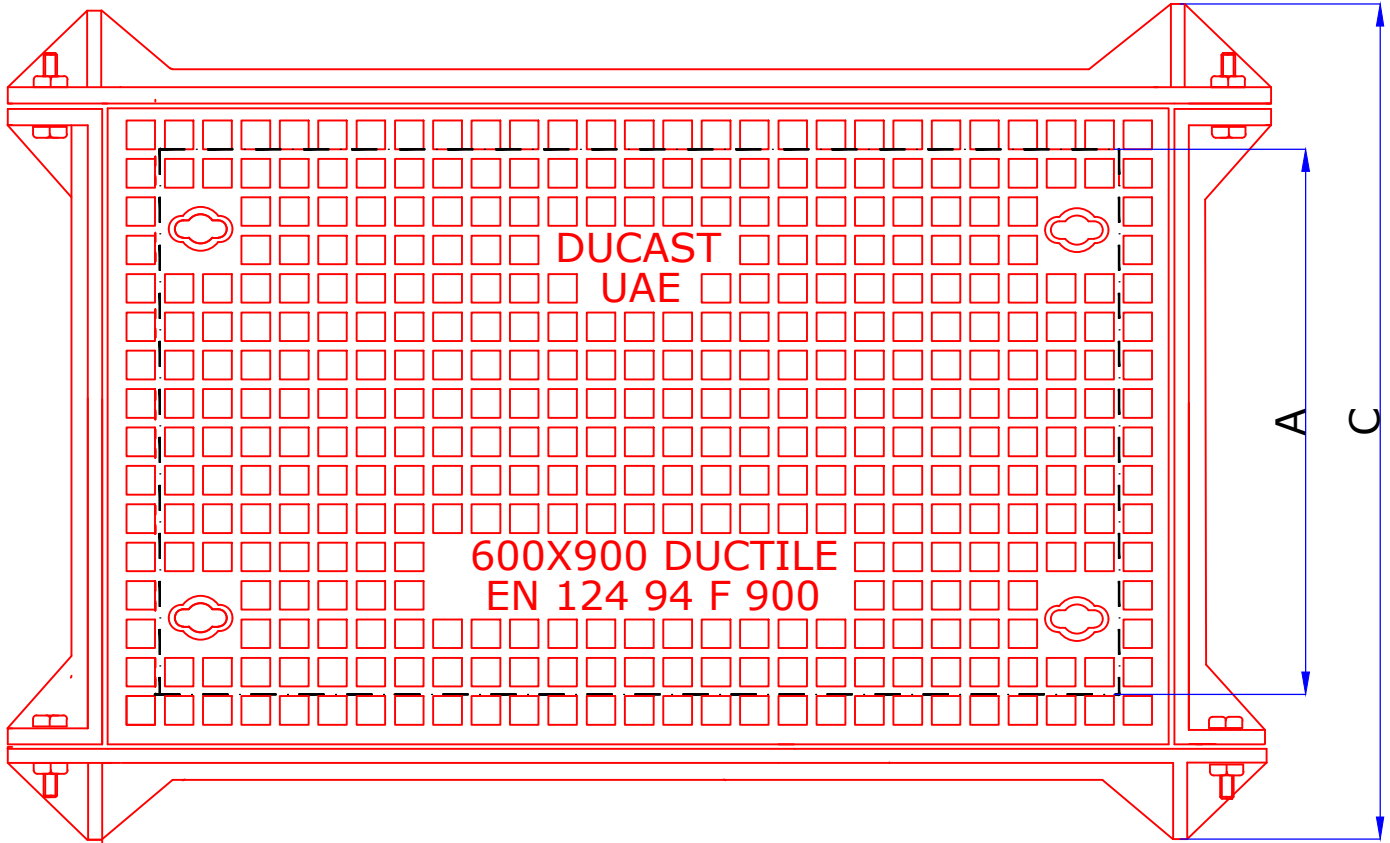
PLAN OF COVER & FRAME
