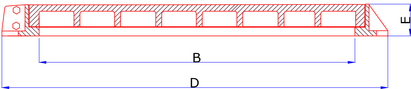
SECTIONAL VIEW OF COVER & FRAME
