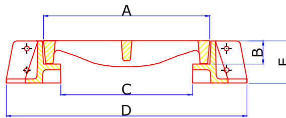
SECTIONAL VIEW
