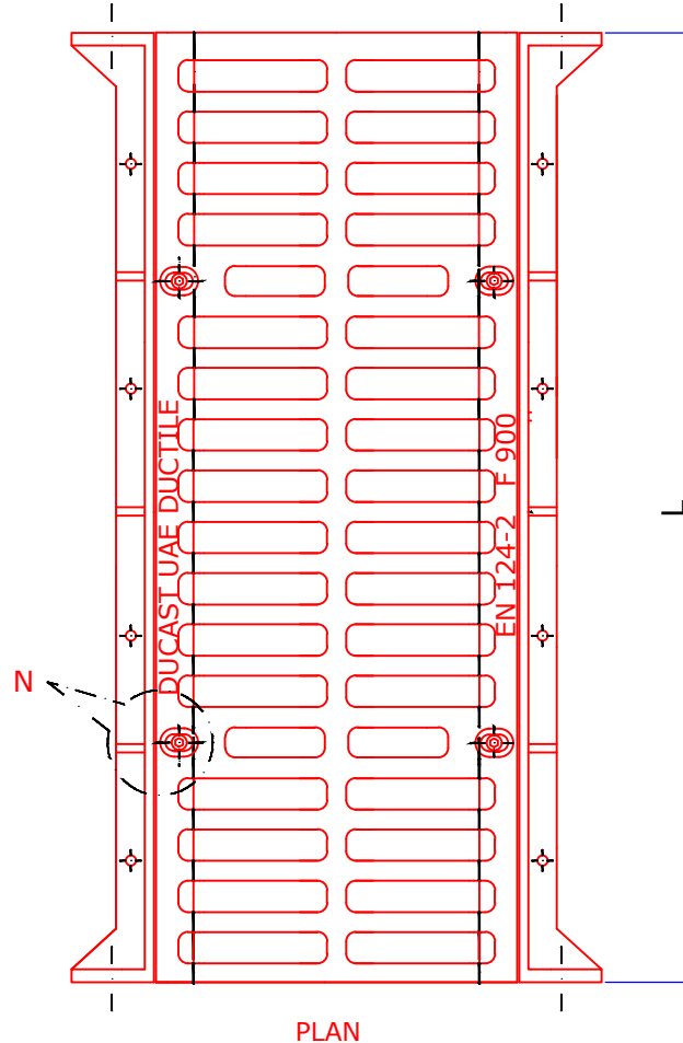
PLAN
