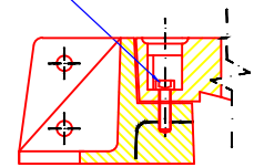
SECTION M-M
