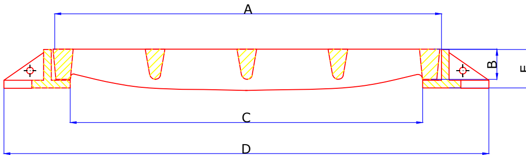
SECTIONAL VIEW
