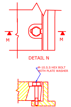
SECTION M-M
