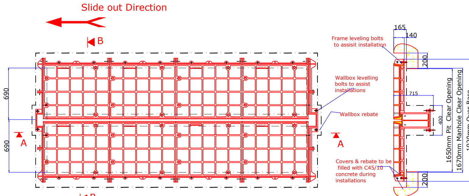
Plan View of Cover & Frame
