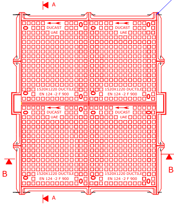
Plan View of Cover & Frame
