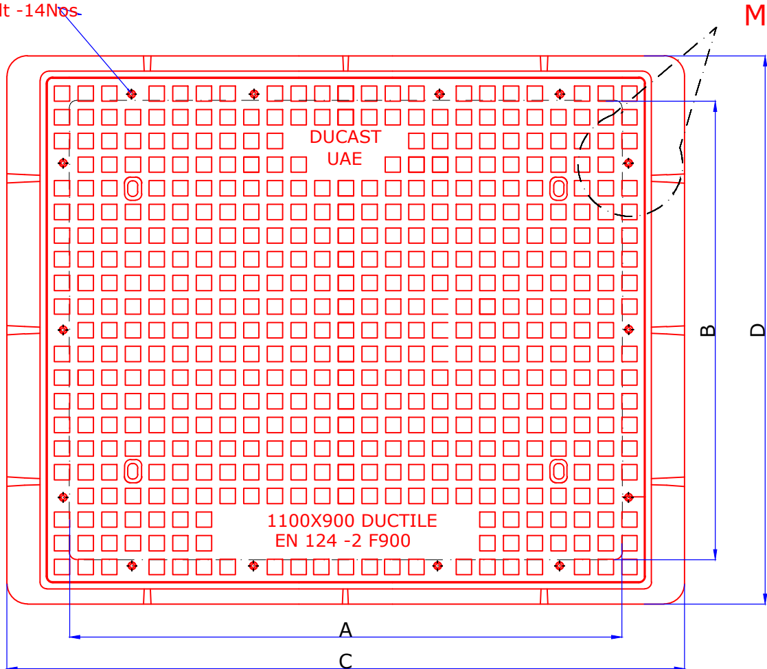
Plan View of Cover & Frame
