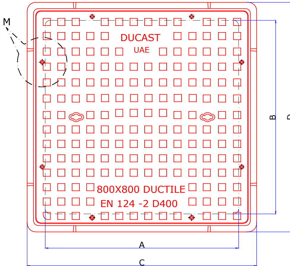
PLAN VIEW OF COVER & FRAME
