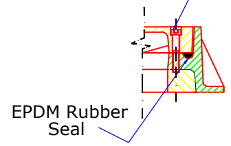
Detail - M
