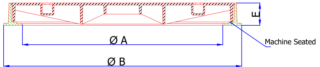
SECTIONAL VIEW OF COVER & FRAME
