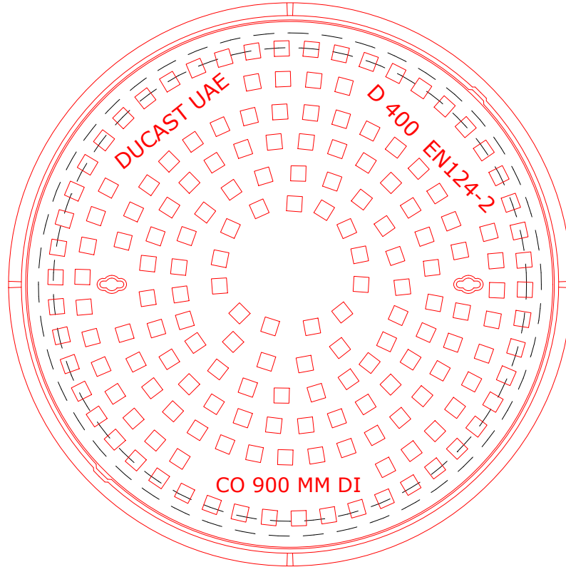
PLAN VIEW OF COVER & FRAME
