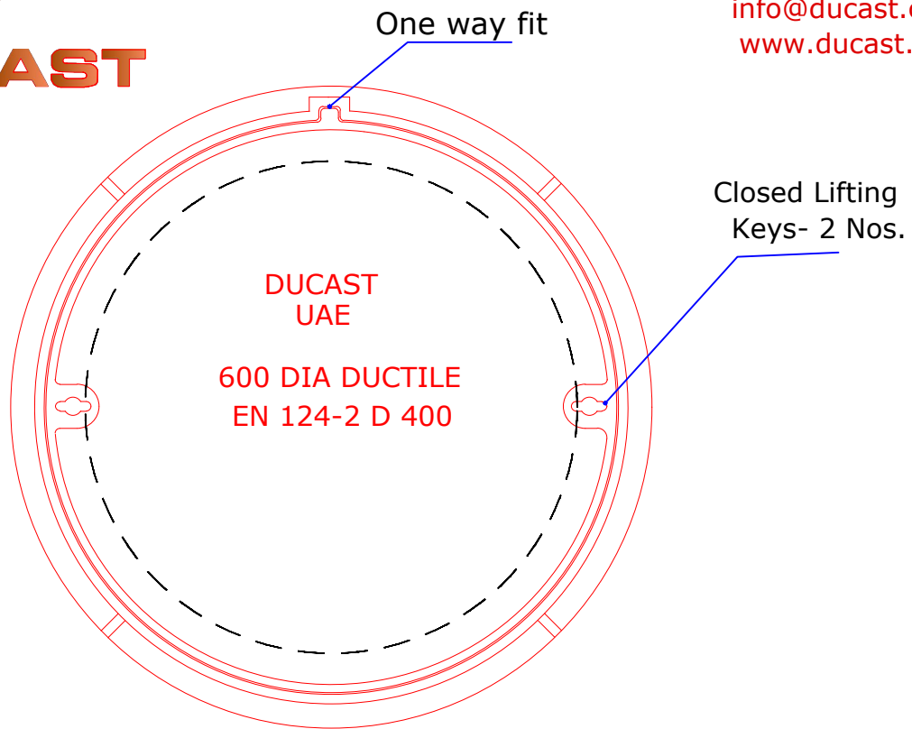
PLAN VIEW OF COVER & FRAME
