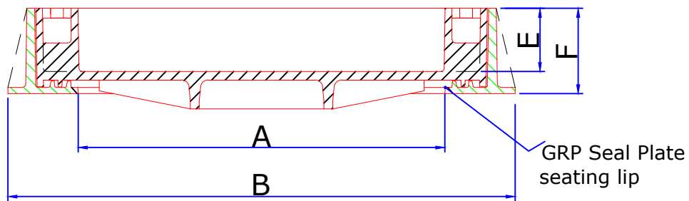
SECTIONAL VIEW OF COVER & FRAME
