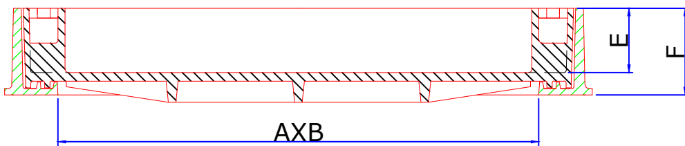
Sectional View of Cover & Frame
