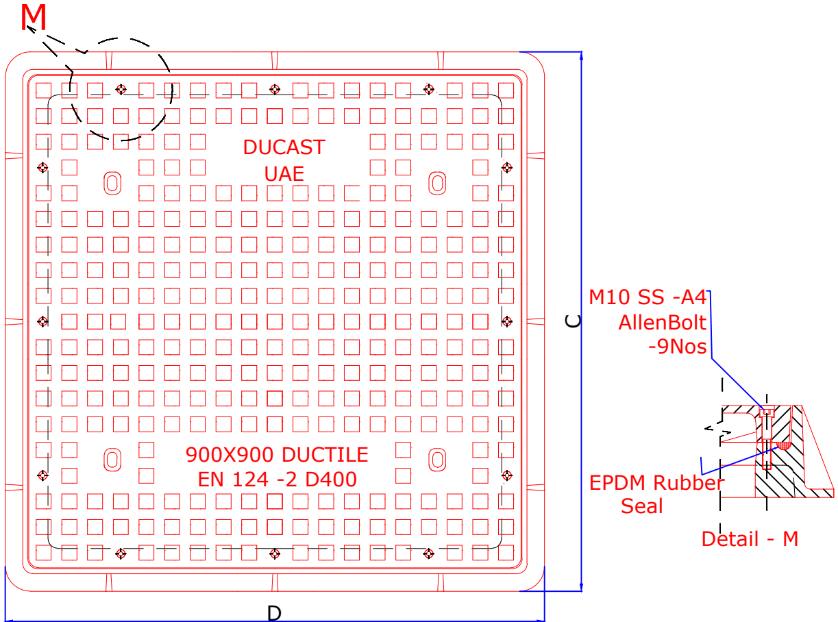
PLAN VIEW OF COVER & FRAME
