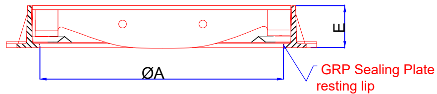
SECTIONAL VIEW
