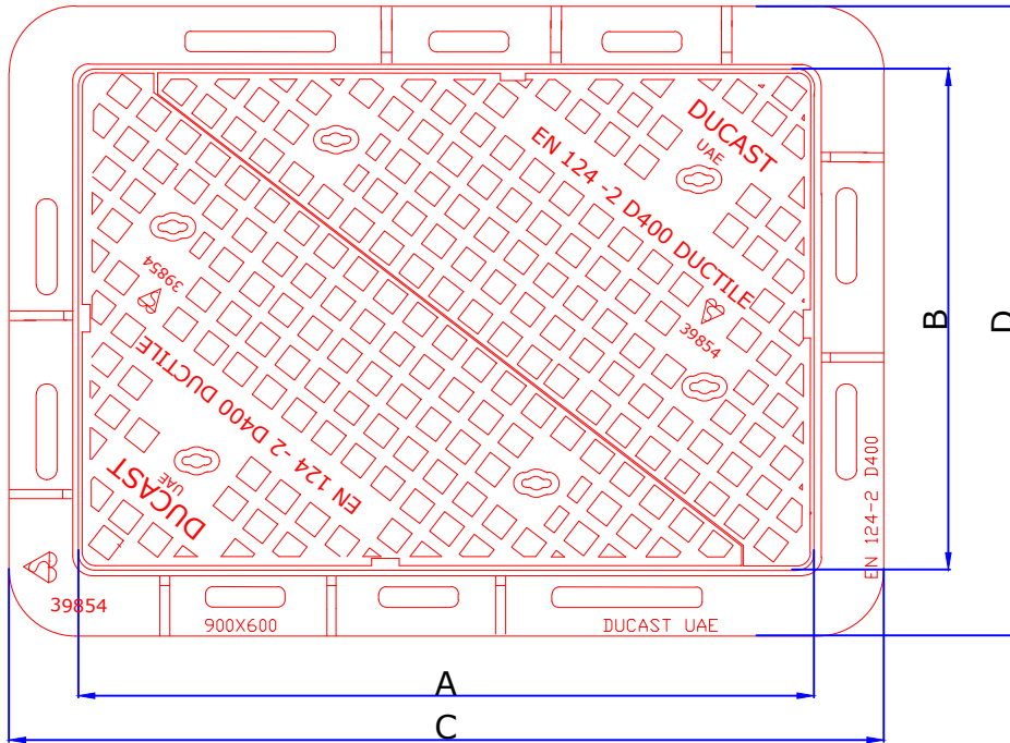
PLAN OF COVER & FRAME
