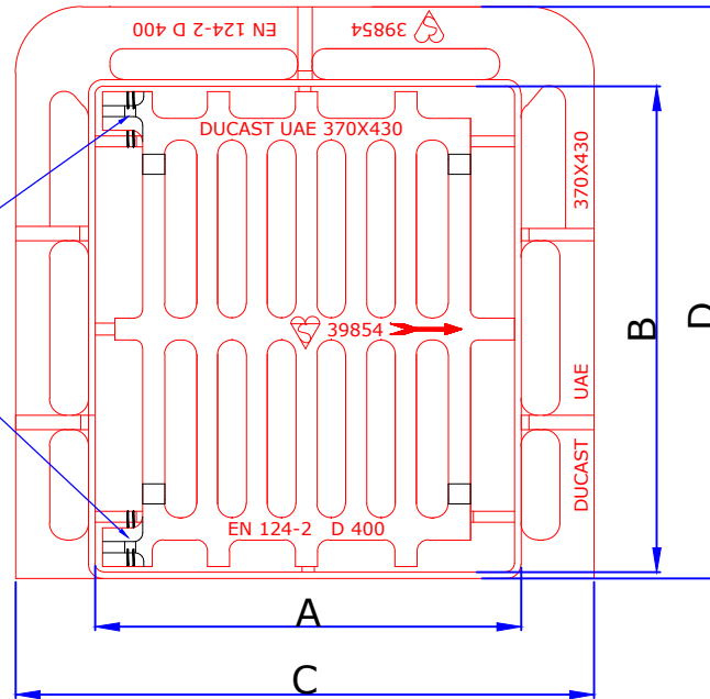
Plan View of Grating & Frame
