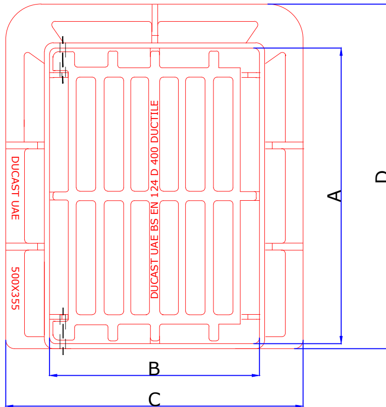
Plan View of Grating & Frame
