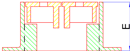
SECTIONAL VIEW OF COVER & FRAME
