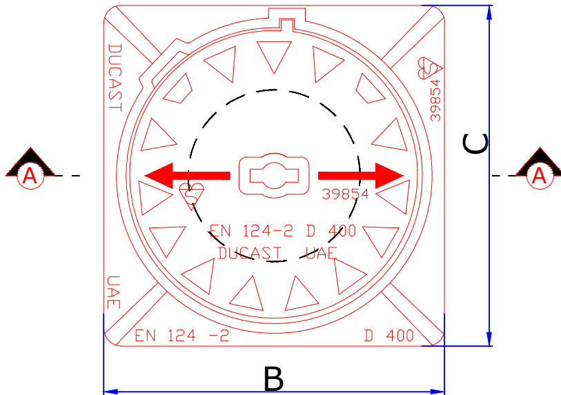
PLAN VIEW OF COVER & FRAME
