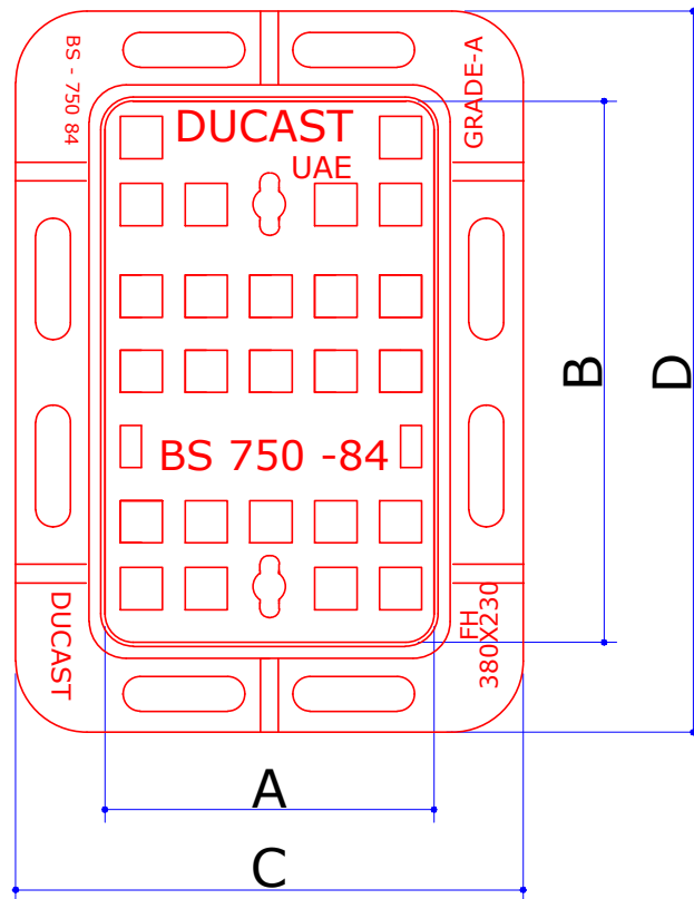
PLAN OF COVER & FRAME
