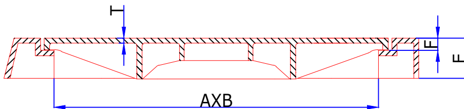
SECTIONAL VIEW OF COVER & FRAME
