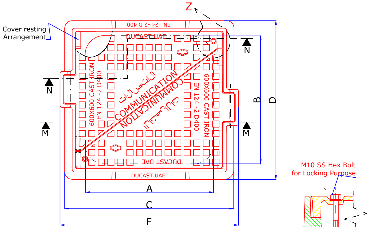
Plan View of Cover & Frame
