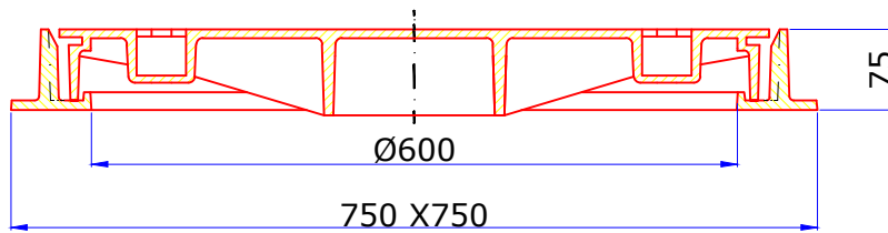
Sectional View of Cover & Frame
