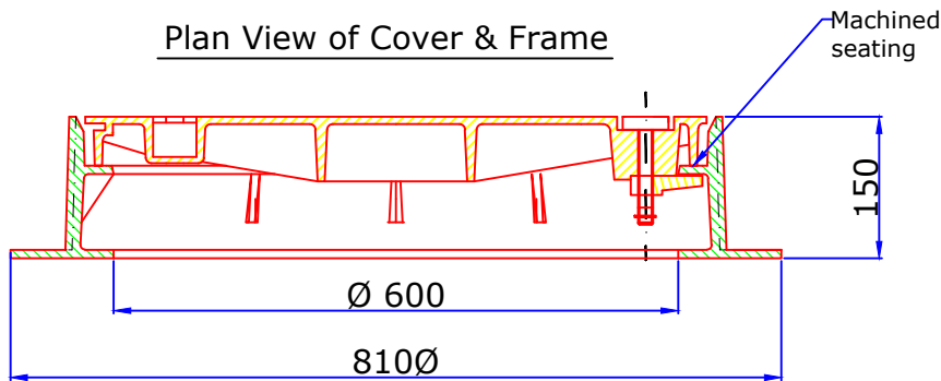
Sectional View of Cover & Frame @ M-M
