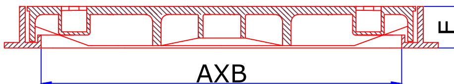
SECTIONAL VIEW
