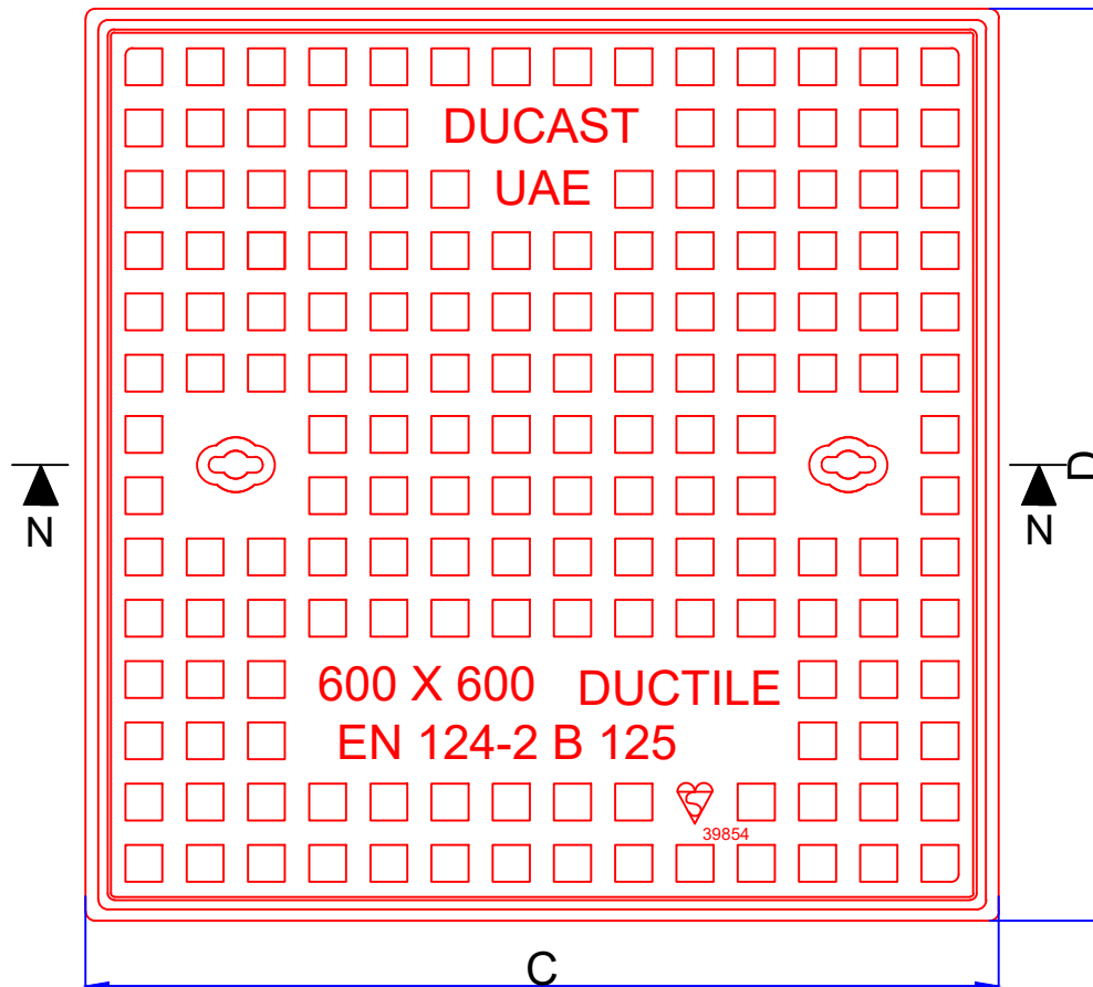
PLAN OF COVER & FRAME
