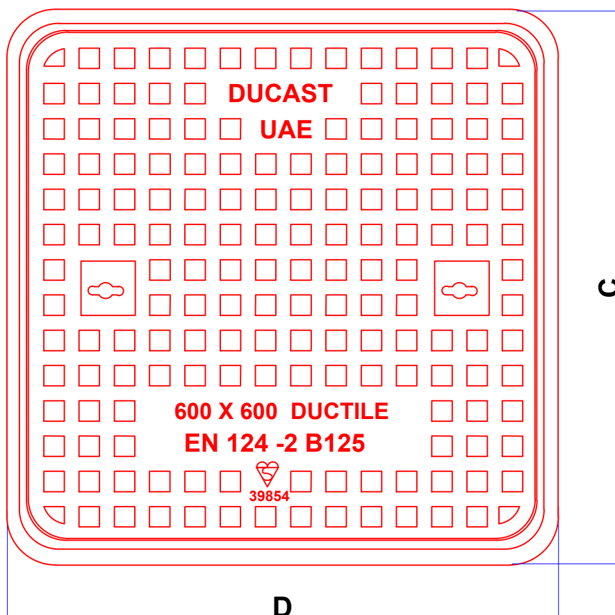
PLAN OF COVER & FRAME
