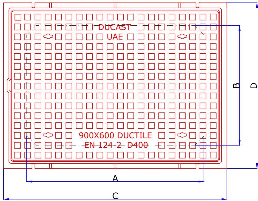
PLAN OF COVER & FRAME
