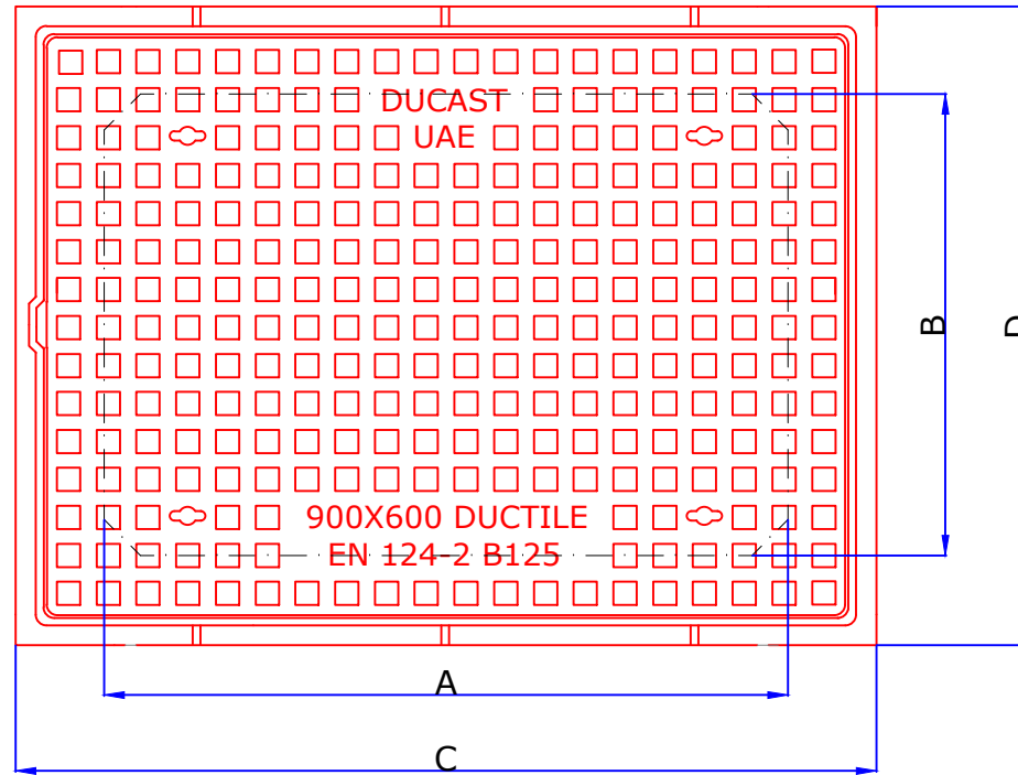
PLAN OF COVER & FRAME
