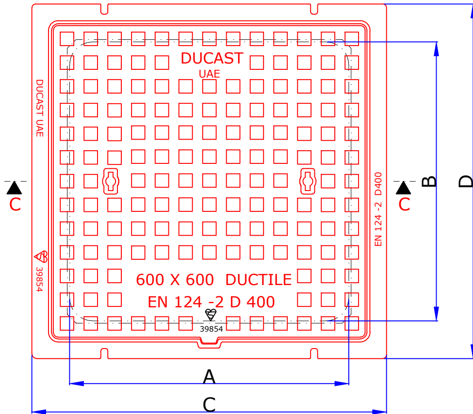
PLAN VIEW OF COVER & FRAME
