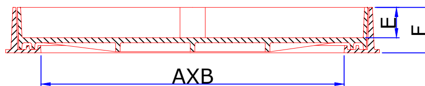
Sectional View of Cover & Frame
