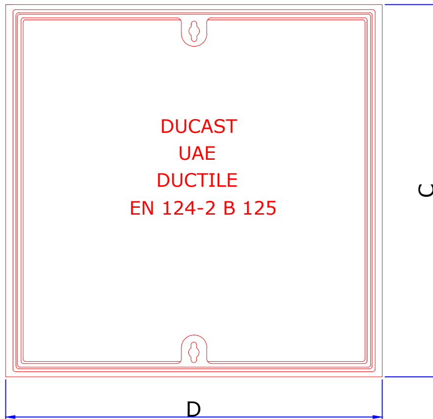
Plan View of Cover & Frame
