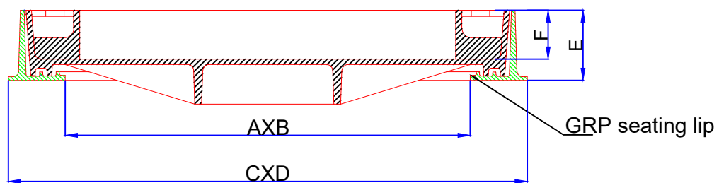
Sectional View of Cover & Frame
