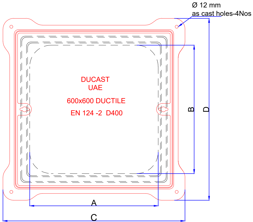
Plan View of Cover & Frame
