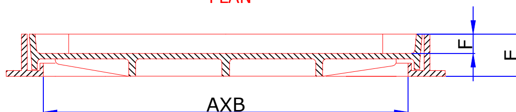
SECTIONAL VIEW
