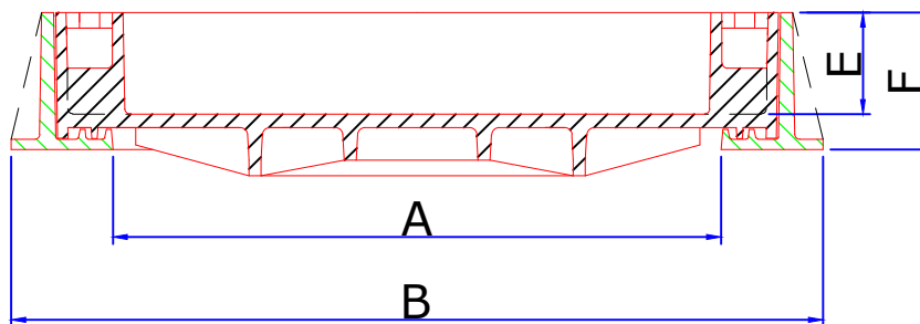
SECTIONAL VIEW OF COVER & FRAME
